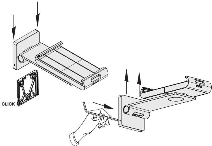
5 | TABLET HOLDER WALL PRO
